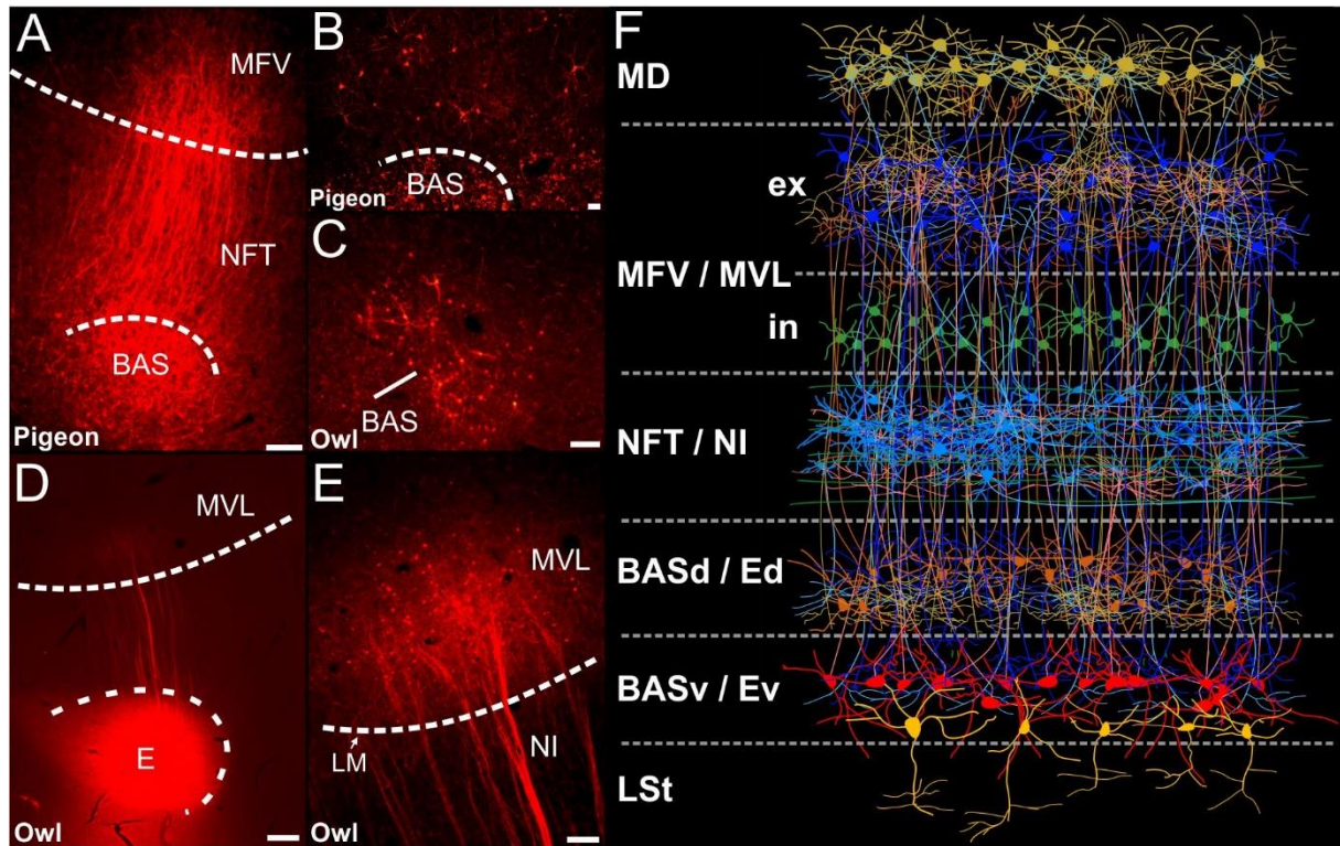
Figure S2: Local connections within DVR. The species is indicated on each figure. (A) Vertically oriented fibers emerging from BAS projecting to overlying mesopallium. (B) Injections into BAS also labelled neurons in NPT. (C) Retrogradely labelled neurons in BAS after MFV injection. (D) Injection into E in the barn owl with columnar fibers extending into MVL. (E) Fibers and retrogradely labelled neurons in MVL after E injection in the barn owl. (F) Highly schematized depiction of local connections in the trigeminal and visual DVR. Scale bar = 100 \mu m in A, D; 50 \mu m in B; Scale bar =100 \mu m in E.
