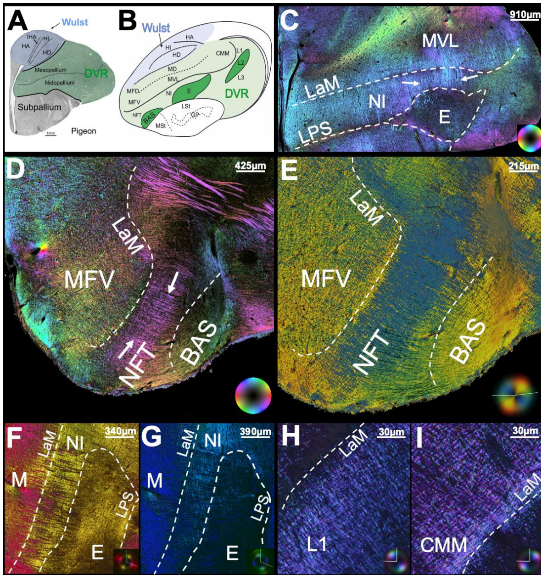
Figure 1) 3D fiber architecture of DVR . A) Schematic localization of hyperpallium (blue) and DVR (green) in frontal and (B) sagittal plane of the pigeon's telencephalon. C) 3D-PLI frontal pallial image at
